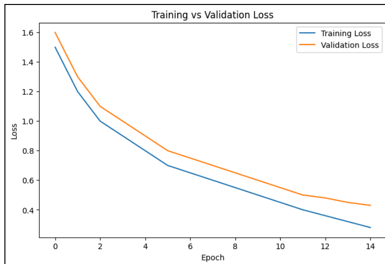
Figure 6: Training and validation loss curves of the AMAE-GCNet model during network optimization.
